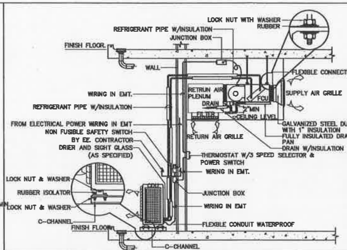
SPLIT TYPE AIR CONDITIONING UNIT INSTALLATION DETAIL
