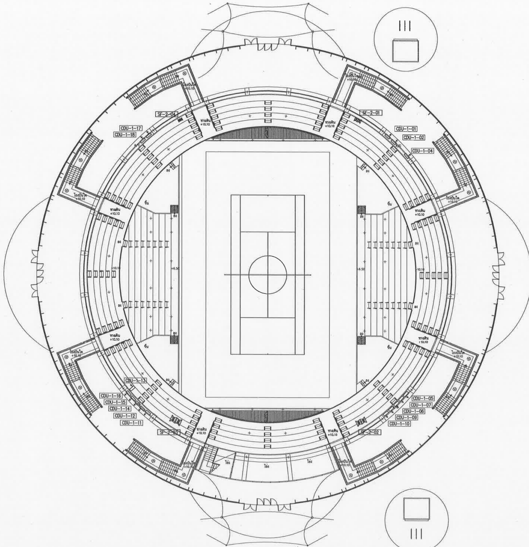
POWER SUPPLY FOR A/C 2nd PLAN
