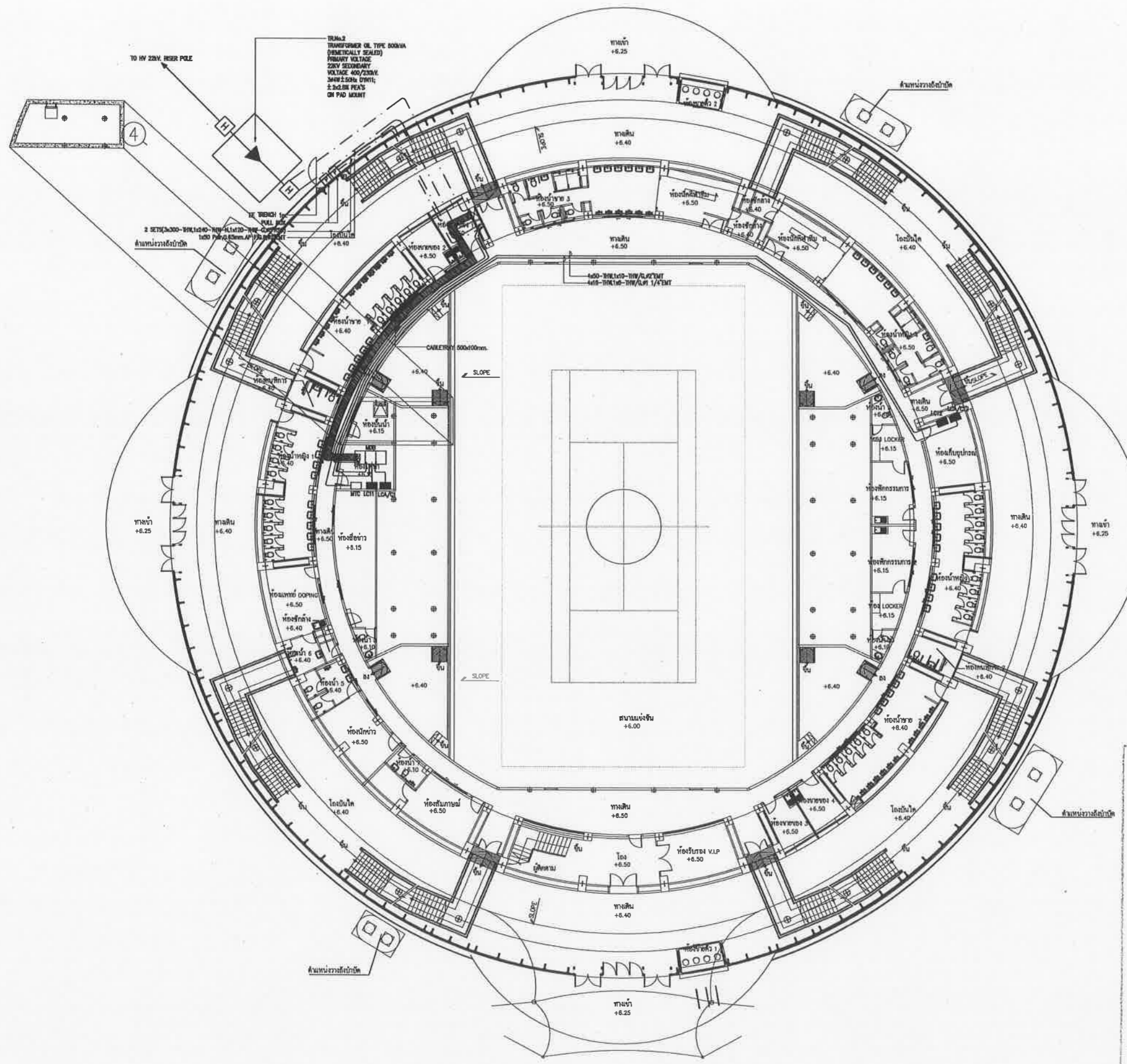
ELECTRICAL POWER FEEDER SYSTEM 1st PLAN
